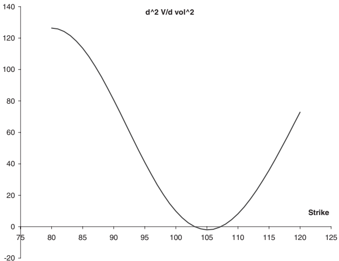
Figure 2-10: \partial^2 V / \partial \sigma^2 versus strike.
