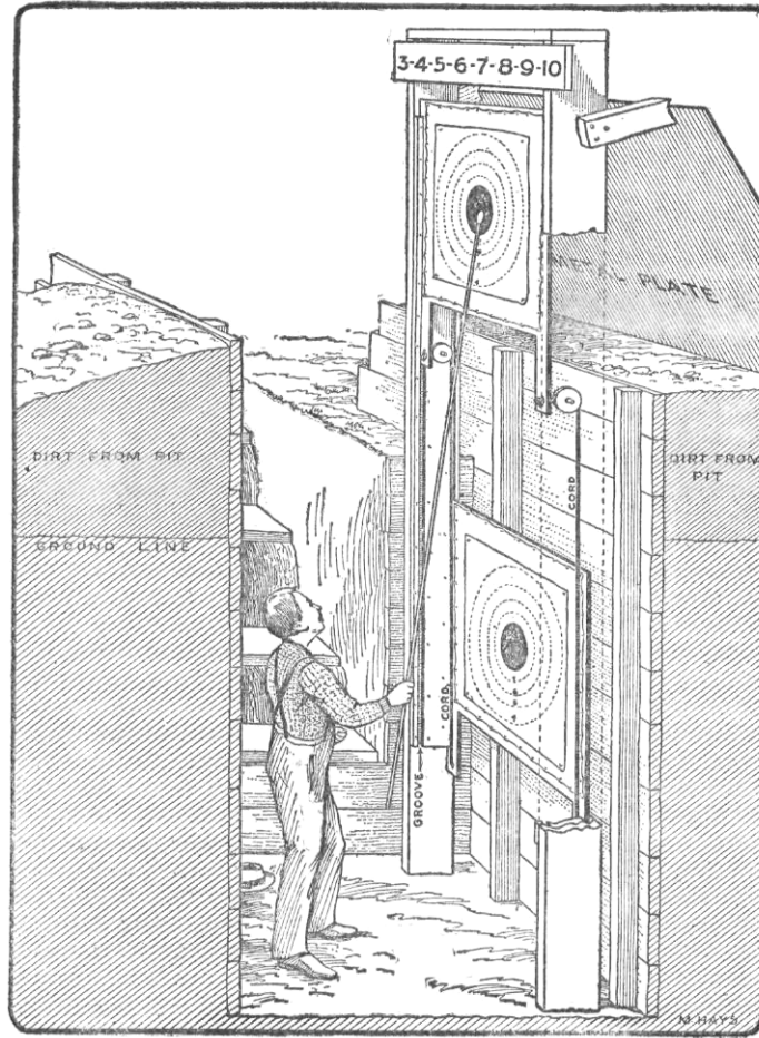
Figure 81 Details of Alternating Targets, Pit. etc., for 50-Yard Range.
